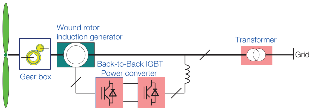
Figure 3-8 – Topology of a doubly fed induction generator (SGCC)
