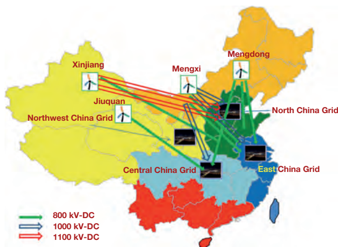
Figure 4-7 – UHVDC transmission plan for some 10 GW-level wind power bases in China (SGCC)
