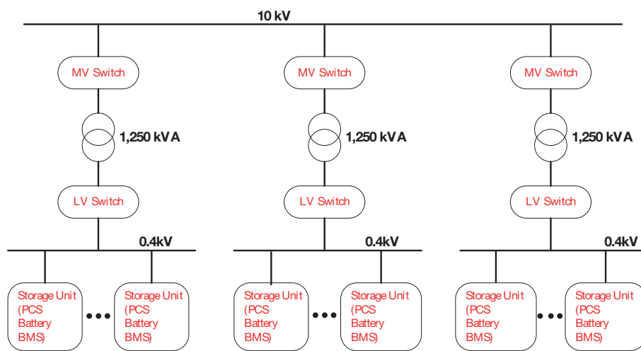
Figure 5-3 – Architecture of the Biling energy storage station (BYD)
