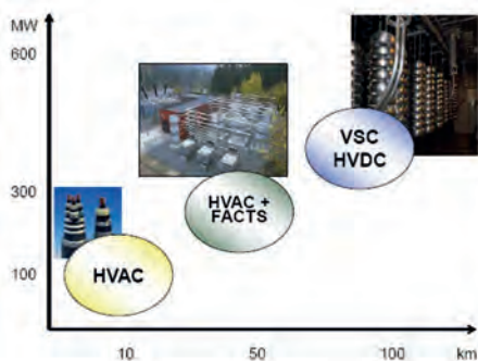
Figure 4-11 – Transmission technologies for integrating offshore wind power [ern11]
