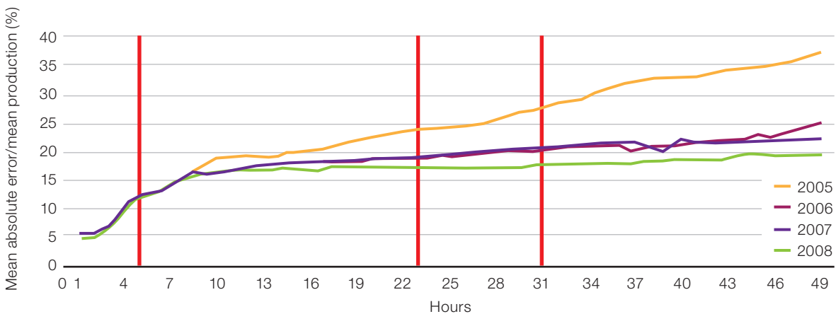
Figure 3-21 – Wind forecast error as a percentage of wind production, as a function of the time forward from the present
