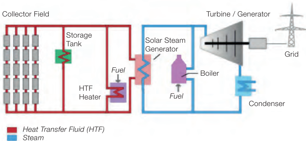
Figure 3-16 – Hybrid CSP plant [gre12]
