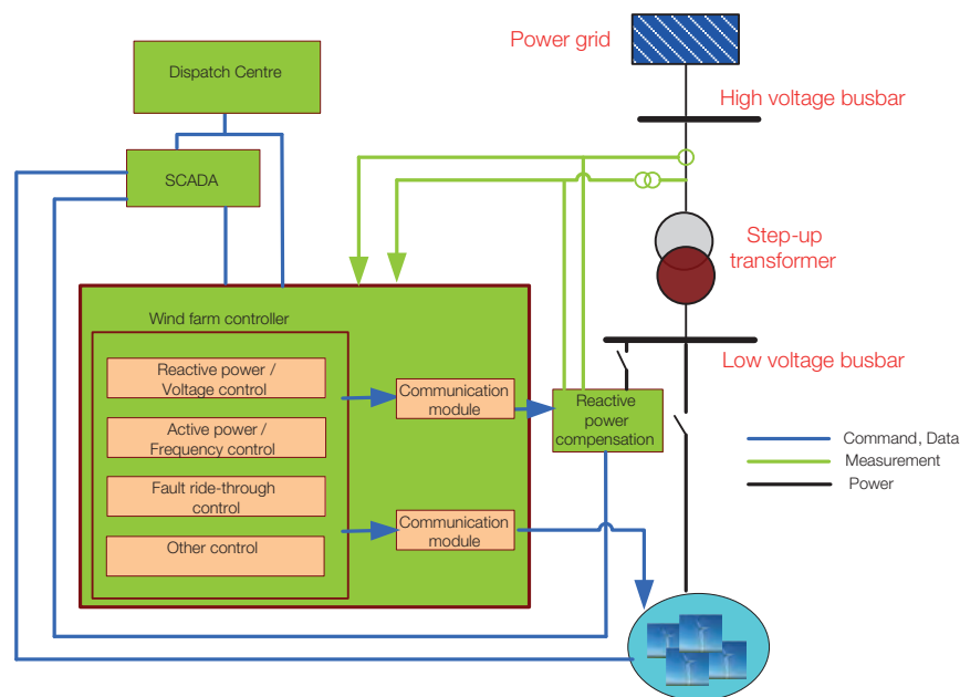
Figure 4-2 – Typical structure of a “grid-friendly” wind power plant (SGCC)
