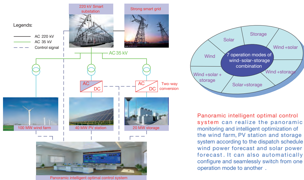
Figure 5-2 – Architecture of the national wind power, solar power, energy storage and transmission demonstration project, Phase I
