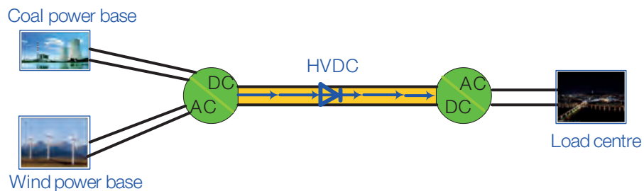
Figure 4-9 – “Wind-fire bundling” design with HVDC transmission (SGCC)
