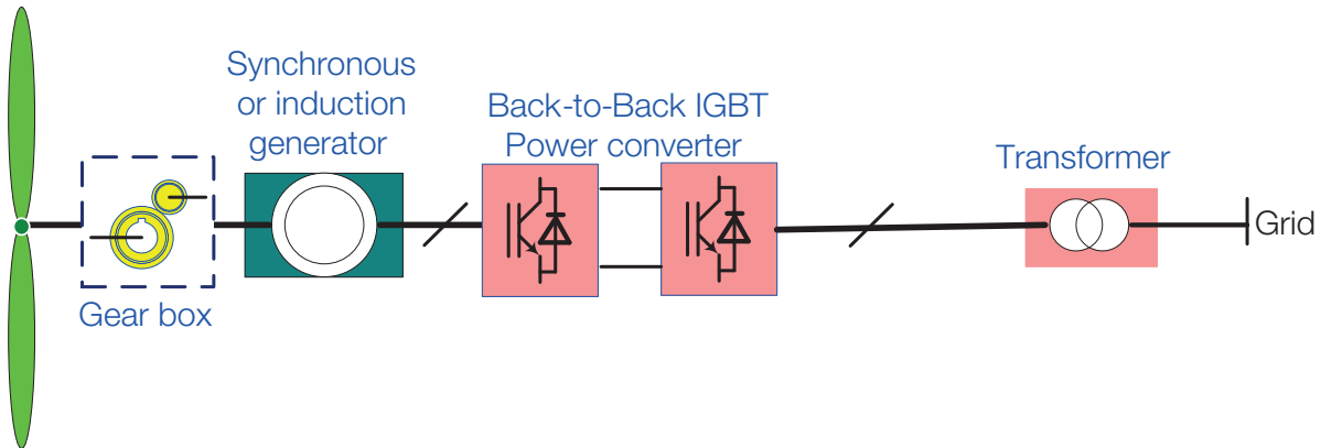
Figure 3-9 – Topology of a full-power conversion WTG (SGCC)
