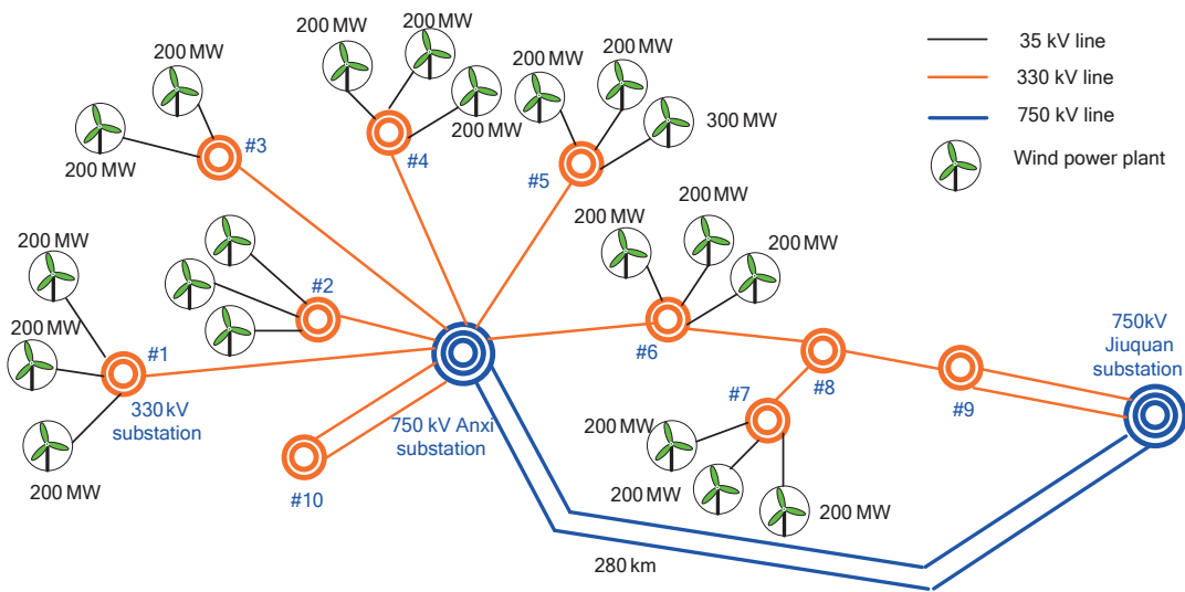
Figure 4-3 – Schematic diagram of the Jiuquan Wind Power Base, Gansu, China (SGCC)
