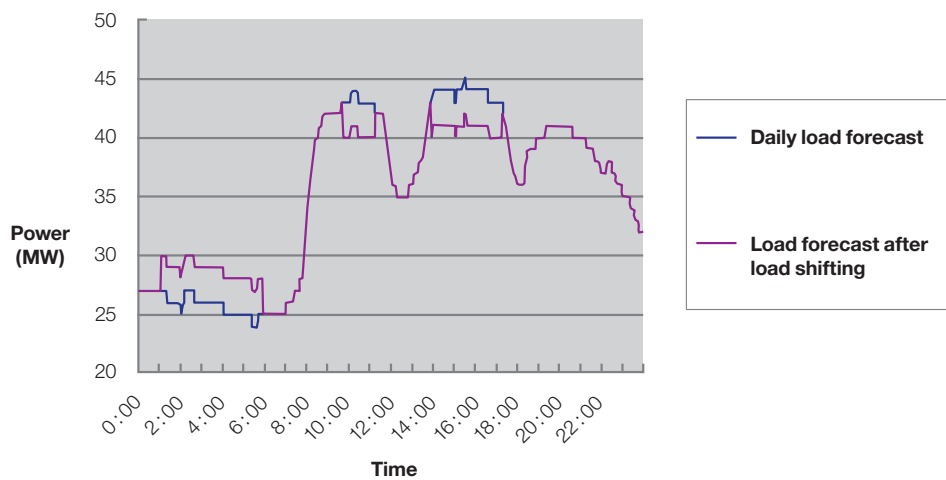
Figure 5-4 – A daily load forecast curve at the Biling substation with/without storage (BYD)
