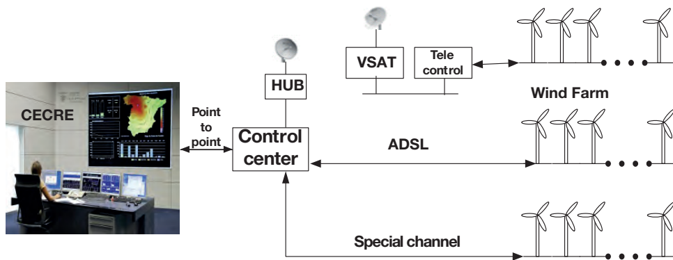
Figure 3-27 – Interconnection between wind farms and CECRE (REE)
