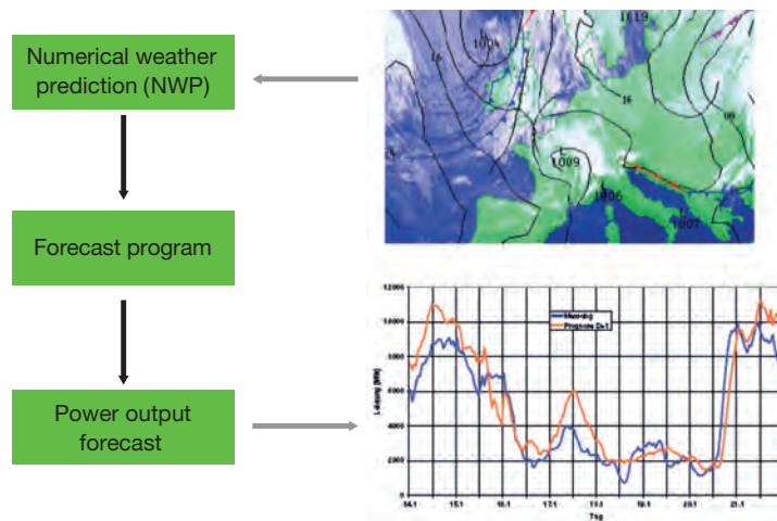
Figure 3-19 – Principle of short-term wind power forecasting (SGCC)
