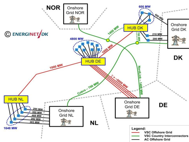
Figure 4-12 – Benchmark test system for the European transnational offshore grid [coc11]
