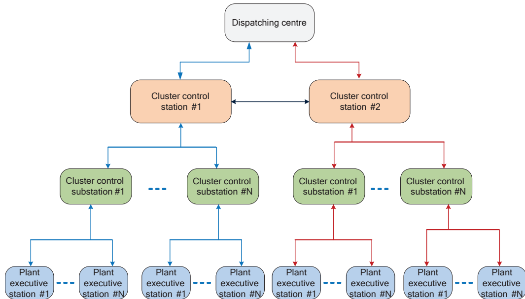
Figure 4-4 – RE power plant cluster control system structure (SGCC)
