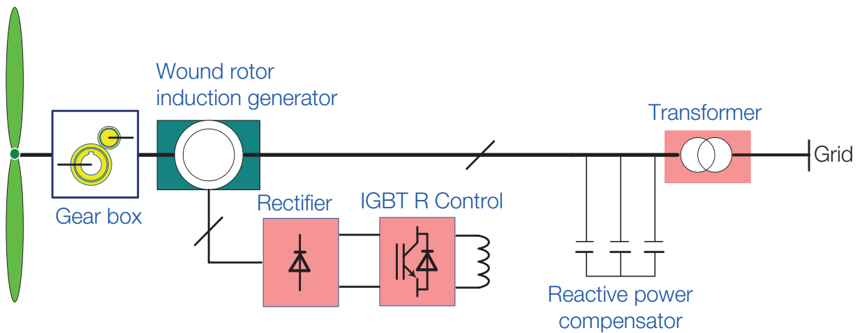
Figure 3-7 – Topology of a variable-slip induction generator (SGCC)
