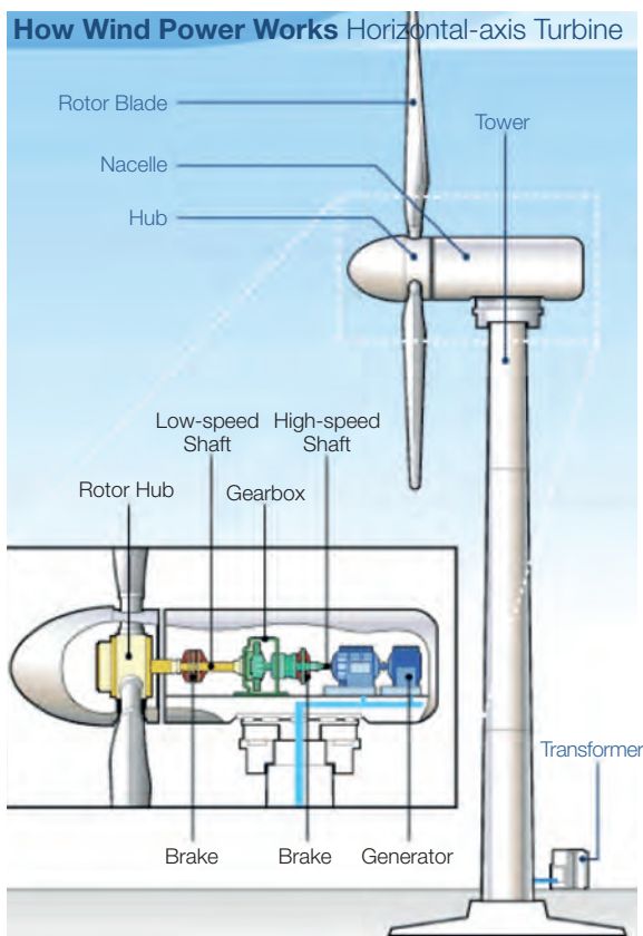
Figure 3-2 – Structure diagram of a WTG (HowStuffworks)
