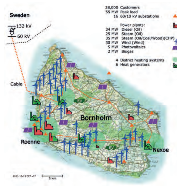
Figure 5-9 – Bornholm’s distribution grid and power plant locations [evf10]
