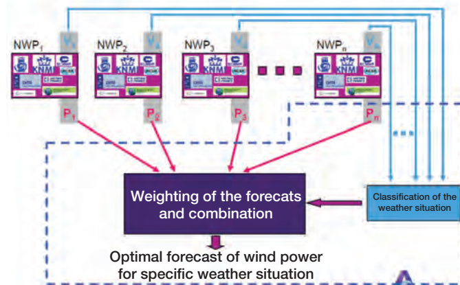
Figure 3-25 – Schematic of a combination tool for wind power forecast (Amprion Company)
