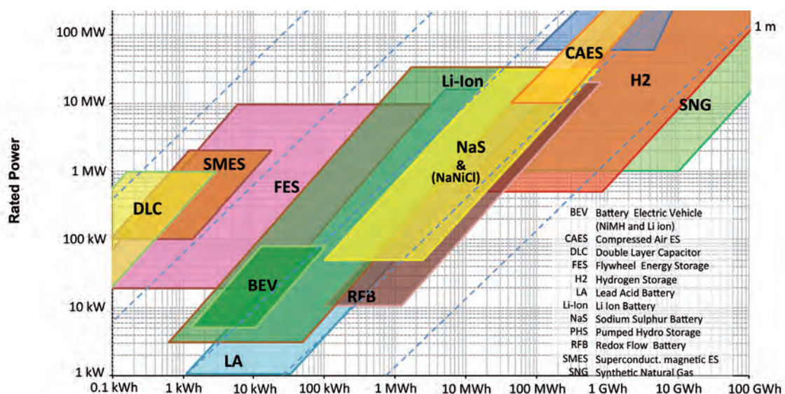
Figure 5-1 – Comparison of rated power, energy content and discharge time of different EES technologies [msb11]
