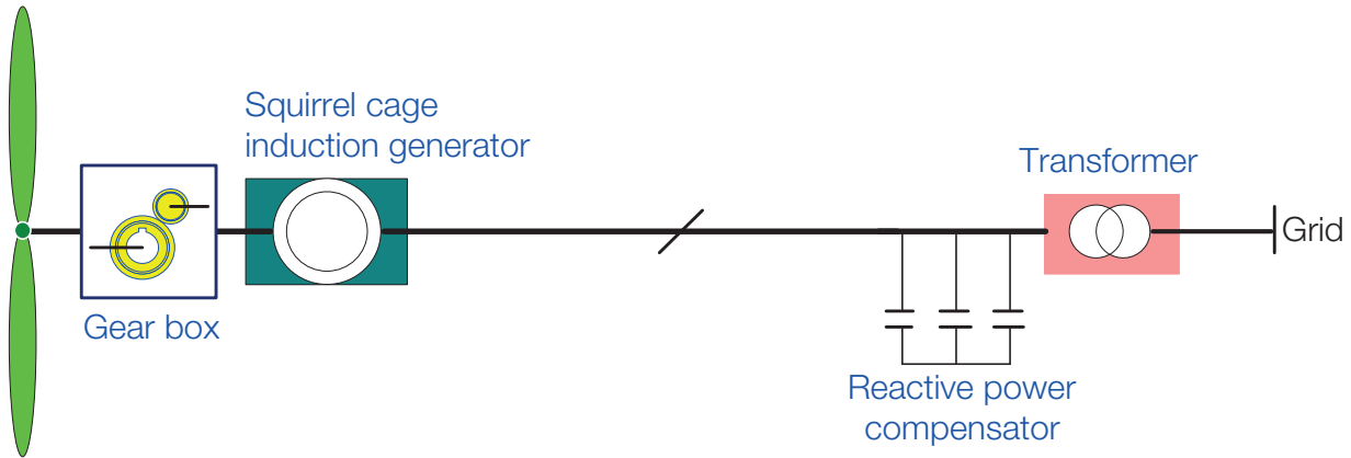
Figure 3-6 – Topology of a fixed speed induction generator (SGCC)
