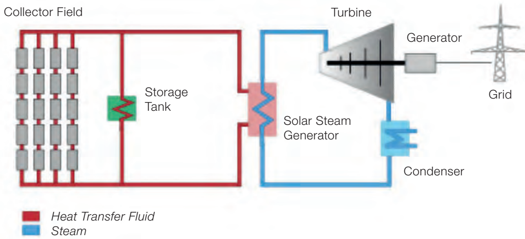
Figure 3-15 – Stand-alone CSP plant [gre12]
