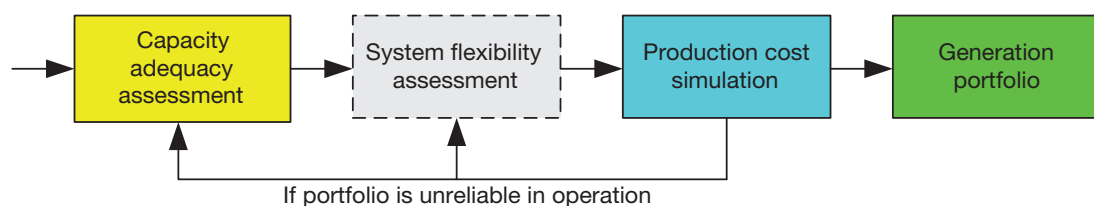
Figure 4-5 – Generation planning process incorporating flexibility assessment
