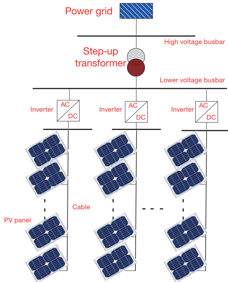
Figure 3-11 – Structure diagram of a PV power station
