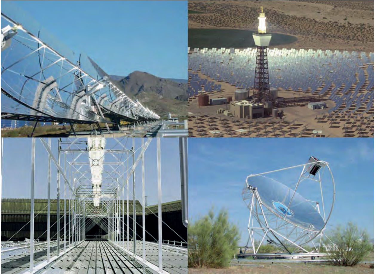
(a) Parabolic trough system (b) Linear Fresnel reflector (LFR)
