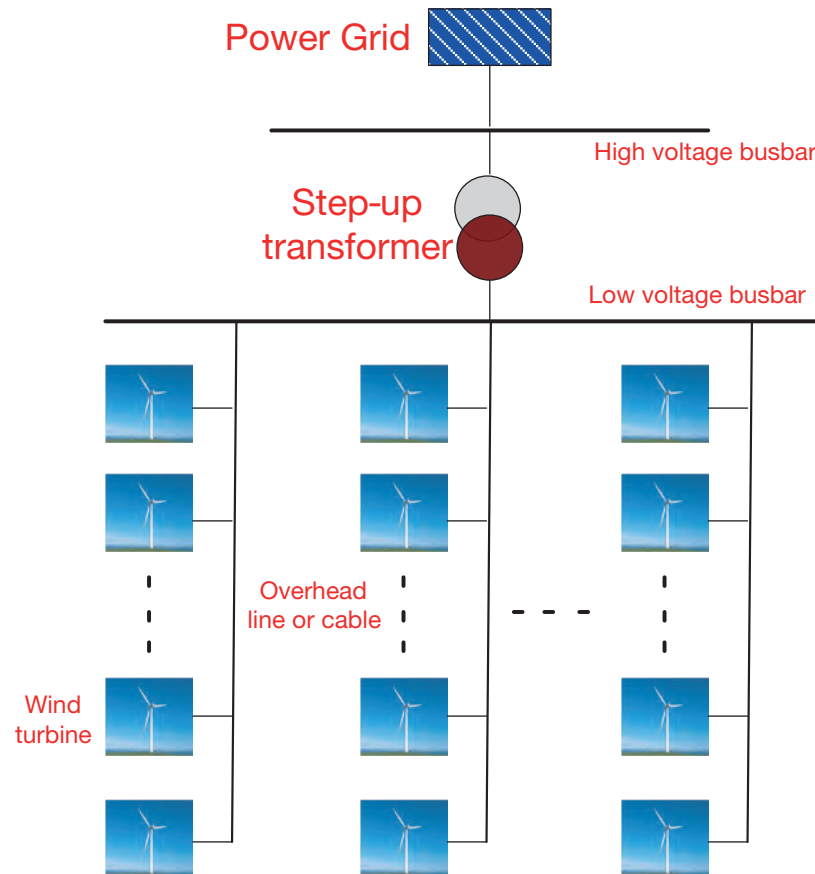
Figure 3-5 – Structure diagram of a wind farm (SGCC)
