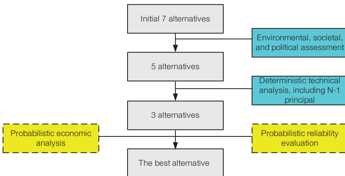
Figure 4-13 – Conceptual flow chart of probabilistic transmission planning [pts11]
