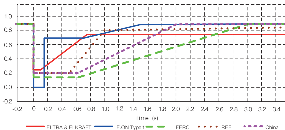
Figure 6-1 – Differences in LVRT requirements in major countries or grid companies (SGCC)
