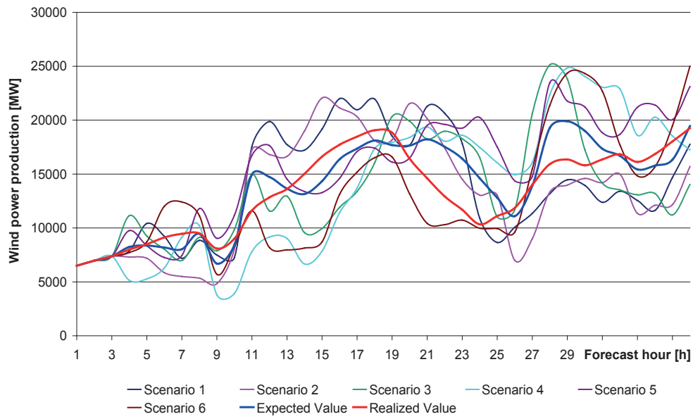
Figure 2-18 – Example of a day-ahead forecast scenario tree for the wind power forecast for the PJM region of the United States [mei10]
