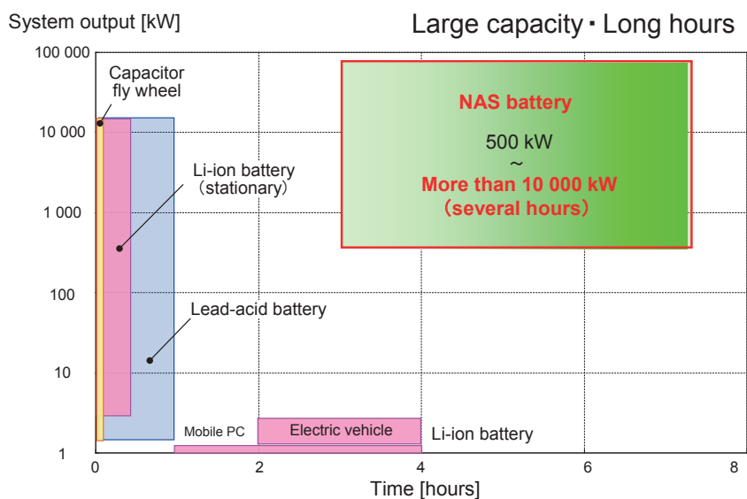
Figure 5-6 – Comparison of battery output and duration (NGK)
