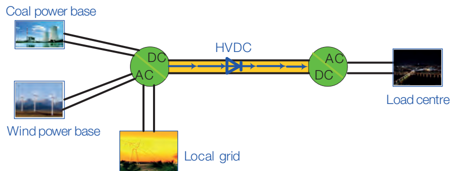
Figure 4-10 – “Wind-fire bundling” design with HVDC transmission and local grid (SGCC)
