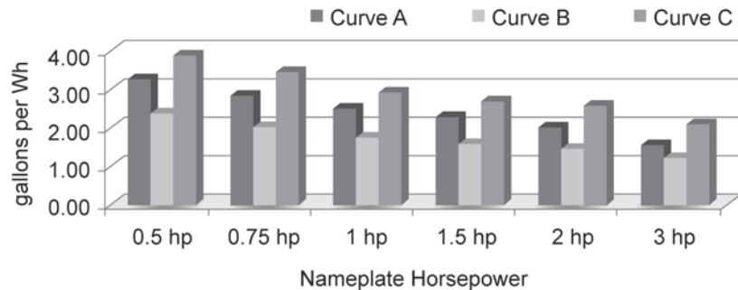
Figure i-1 Energy Factor by HP and System Curves
