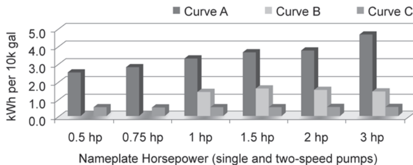
Figure i-2 Horsepower and Speed
