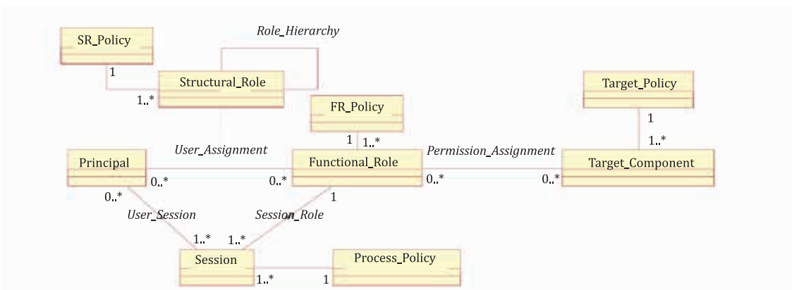
Figure 3 — Policy-driven RBAC Schema
