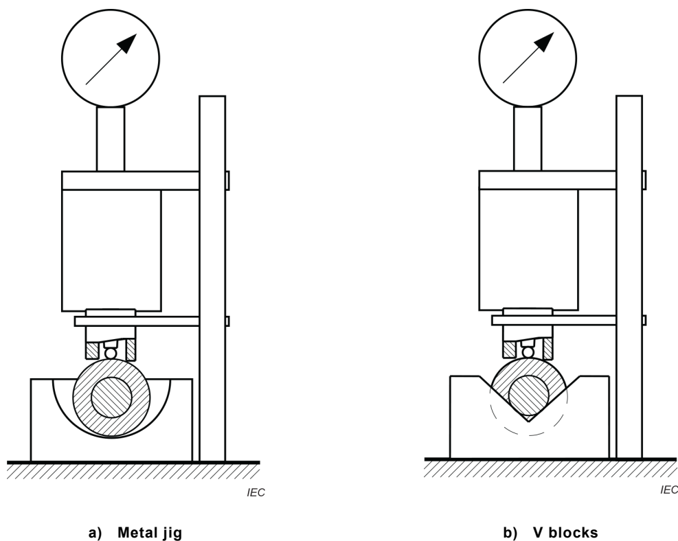
Figure A.2 – Testing surfaces of small radius of curvature
