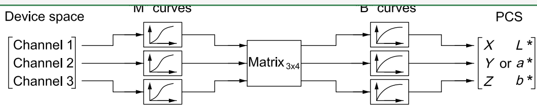
c) Using a lutBToAType model
