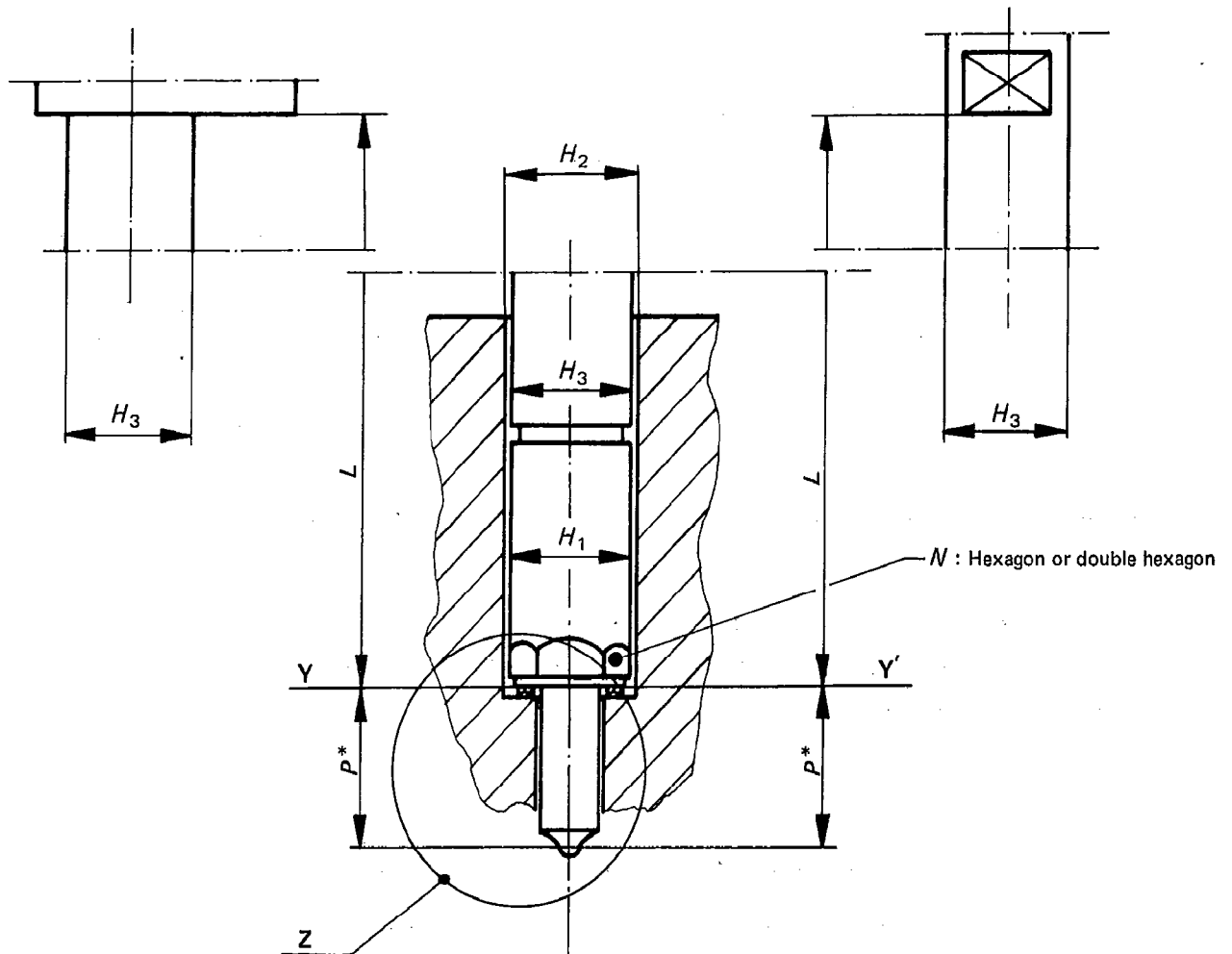
FIGURE 1 – Injection nozzle holder with body, types 8 and 10
