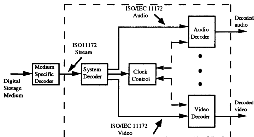
Figure 1 -- Prototypical ISO/IEC 11172 decoder
