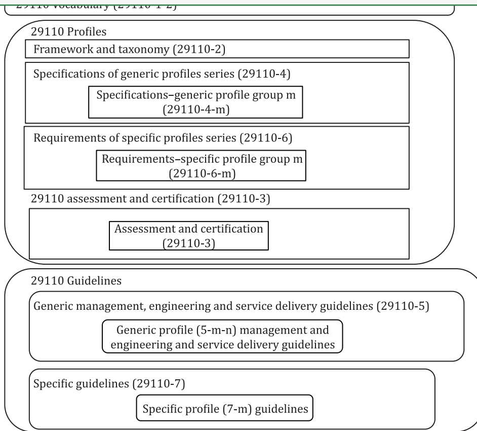
Figure 1 — The ISO/IEC 29110 series
