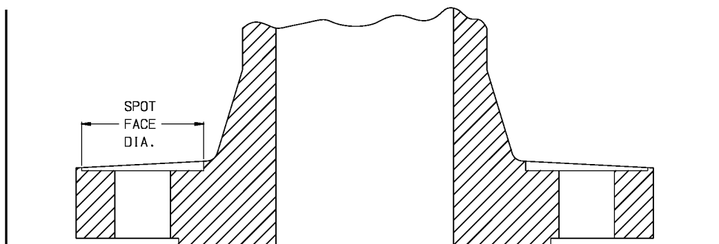
FIGURE 1 Flange with Spot Facing
